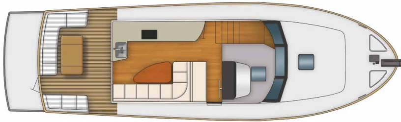
Optional Arrangement with Twin V-berth with 2 day heads
